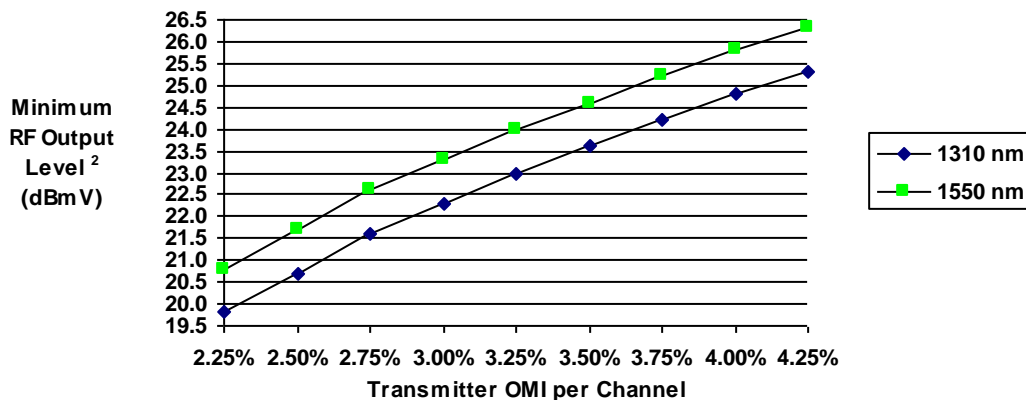
Figure 6. Receiver RF Output Level Vs Transmitter OMI
