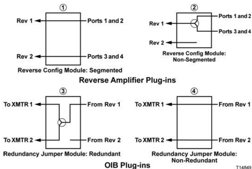
Figure 5. Configuration Module Block Diagram
